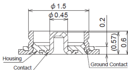
Sect. A-A
