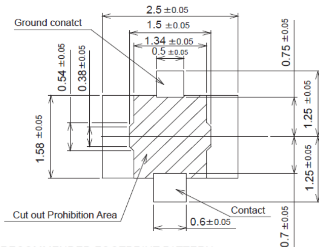
RECOMMENDED FOOTPRINT PATTERN
