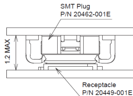
MATED VIEW
